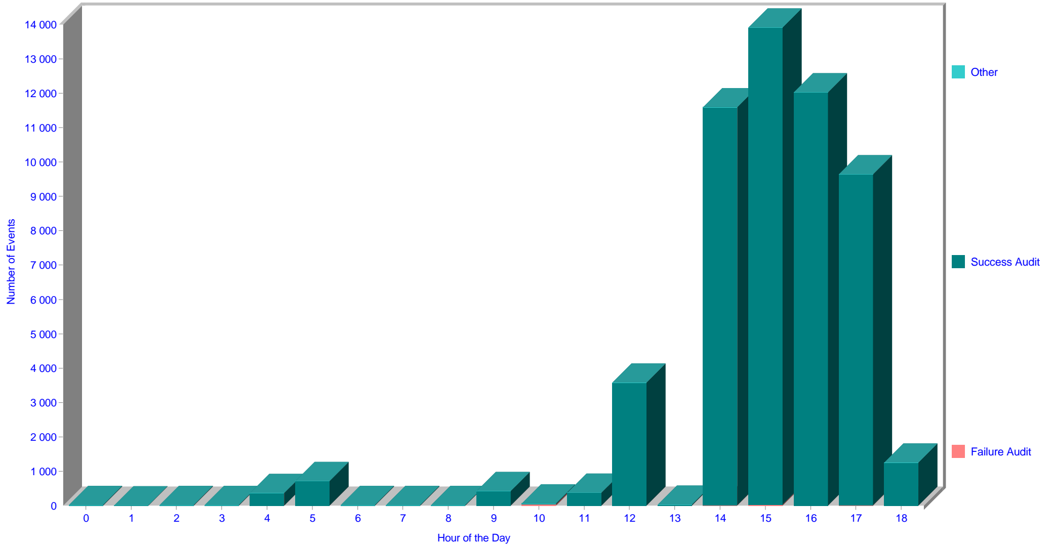
Security Log Activity by Hour of the Day
