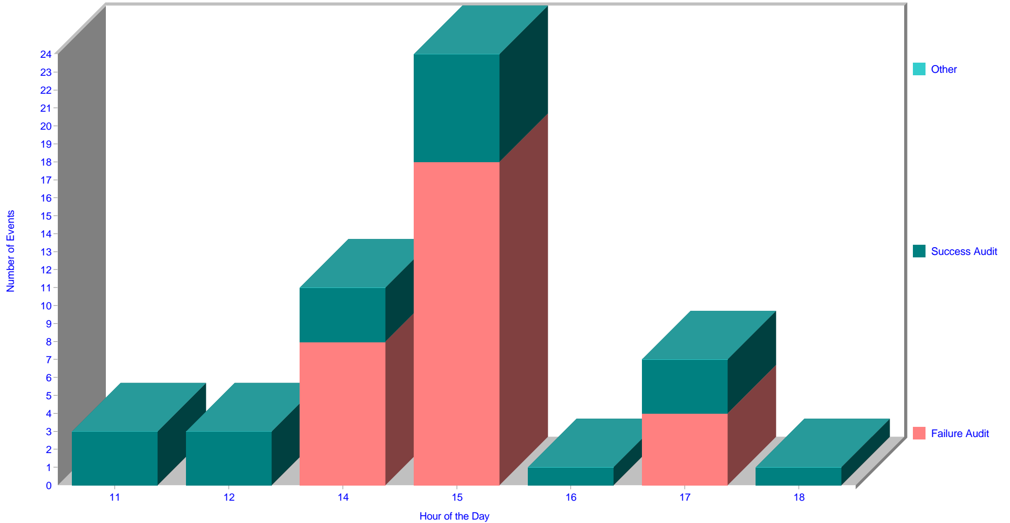
Security Account Logon Activity by Hour of the Day
